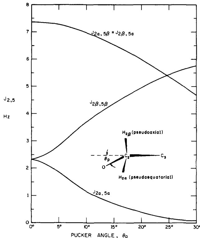
Figure 1. Plots of calculated values of J_{2\alpha,5\beta} = J_{2\beta,5\alpha} , J_{2\alpha,5\alpha} , and J_{2\beta,5\beta} in 2,5-dihydrofuran (1, X = O) as functions of the pucker angle \theta_p in the range 0–30°. The pucker angle and the H \alpha and H \beta are defined schematically in the inset figure in which the C 2 and C 3 carbon atoms eclipse the C 5 and C 4 carbon atoms, respectively.
